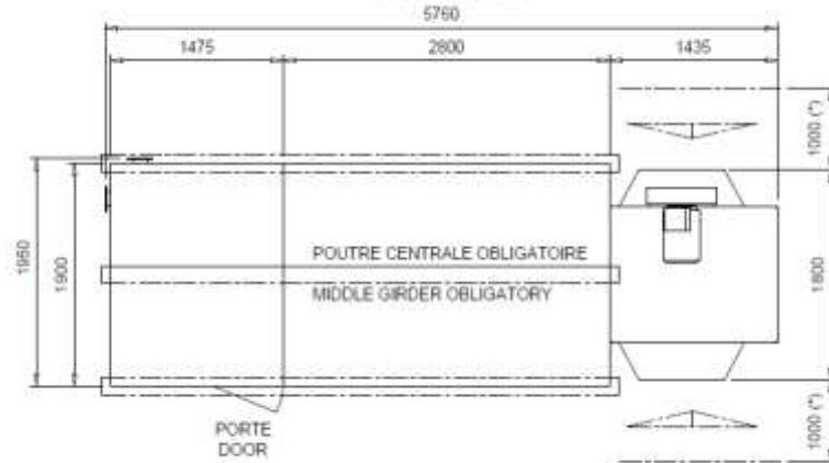
PLAN DE POSE SF2718 SF2718 BASEMENT
