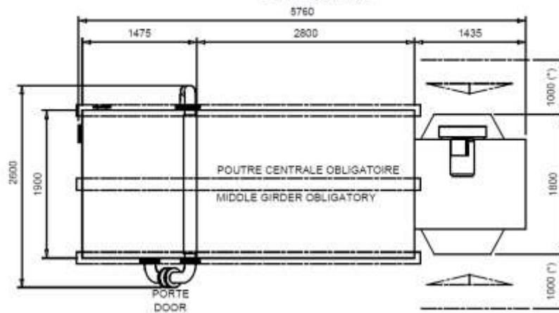
PLAN DE POSE SFIM3021 SFIM3021 BASEMENT
