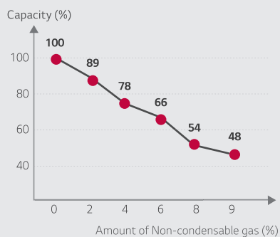
Capacity According to the Amount of Non-condensable Gas
